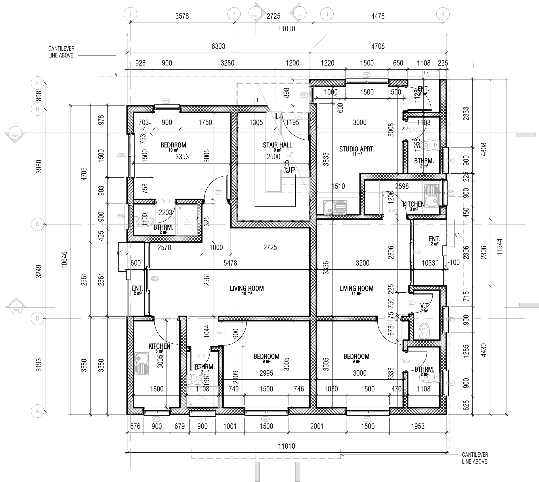
1 GROUND FLOOR PLAN 1 : 75
